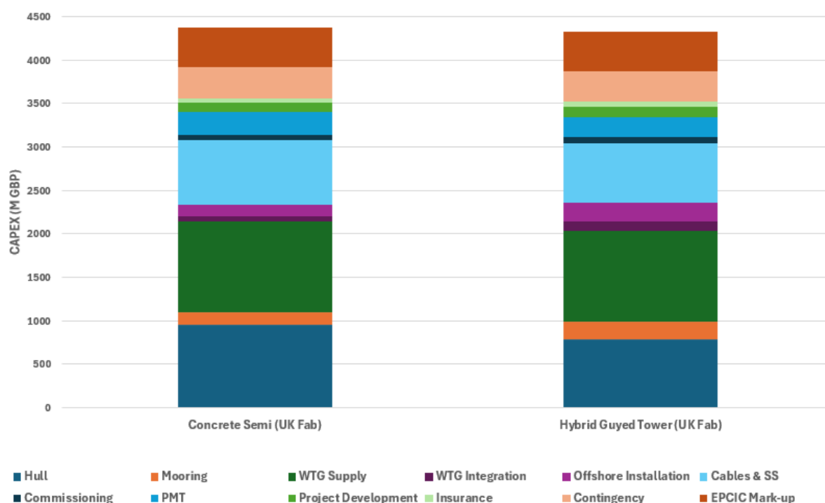
Figure 6.1 CAPEX Comparison (750 MW)
